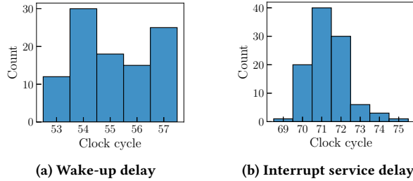
Figure 16: The histogram of the delay in servicing the message request by the energy supervisor in clock cycles.
